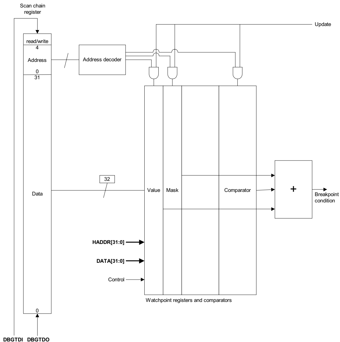
Figure 9-12 EmbeddedICE-RT block diagram
